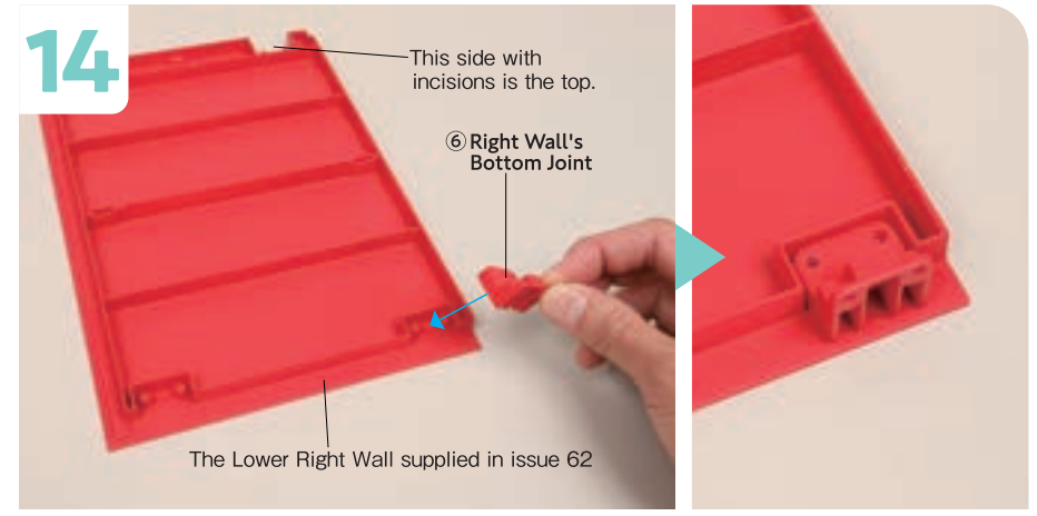
Detach the Lower Right Wall supplied in issue 62 in which we have checked how to assemble, and fit the ⑥ Right Wall's Bottom Joint to the lower inner side of the wall in the position shown.
