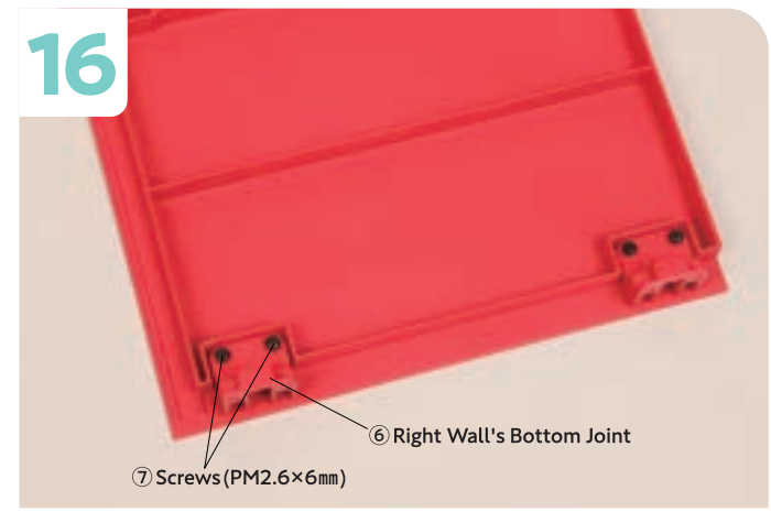
Fit another ⑥ Right Wall's Bottom Joint to the position shown and fix it in place by tightening two ⑦ Screws (PM2.6×6mm) in the same manner.
