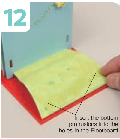
Press the front edge of the Ground against the Floorboard and insert its bottom protrusions into the holes in the Floorboard.
