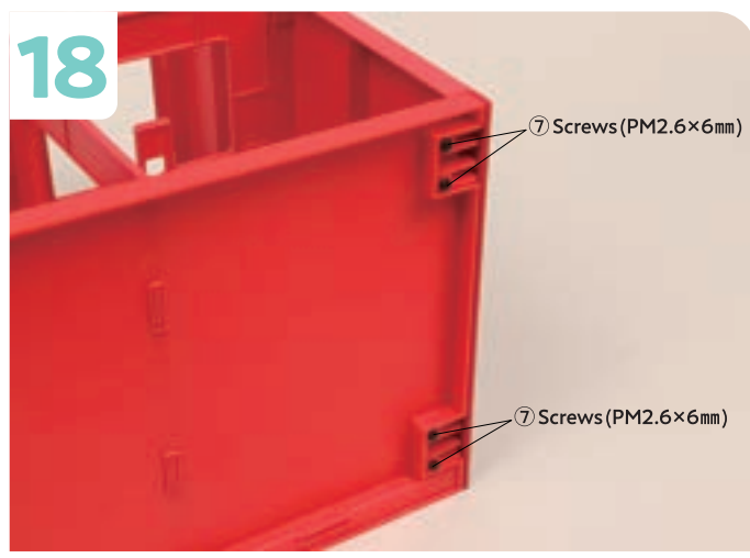
Tighten two ⑦ Screws (PM2.6×6mm) into each Bottom Joint of the Right Wall to fix the wall in place.
